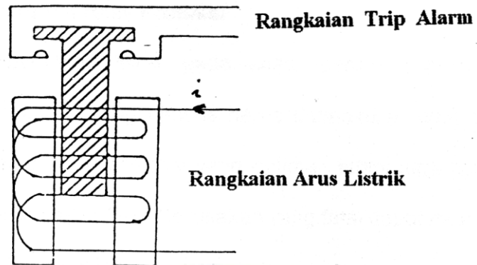
Gambar 2.11 Contoh Relay Listrik
