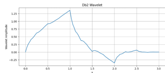
Figure 1: Daubechies Wavelets
