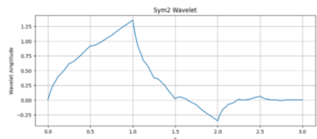
Figure 3: Symlet Wavelets
